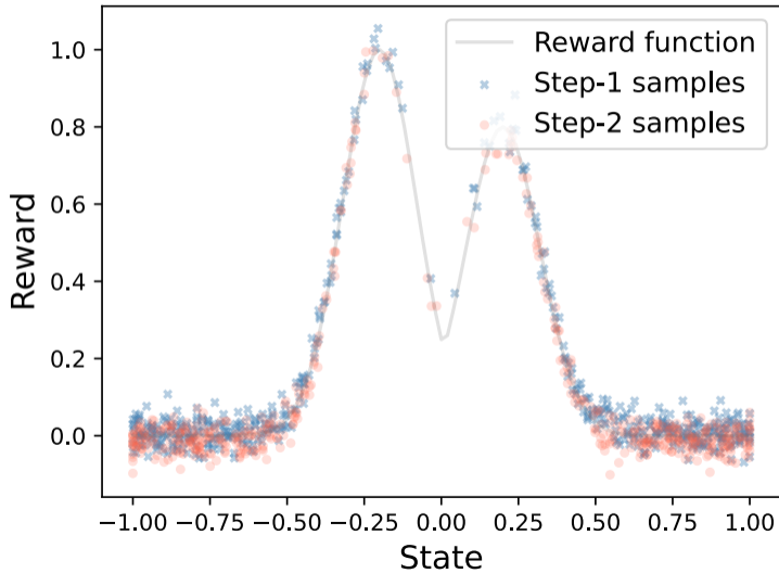
Offline dataset
