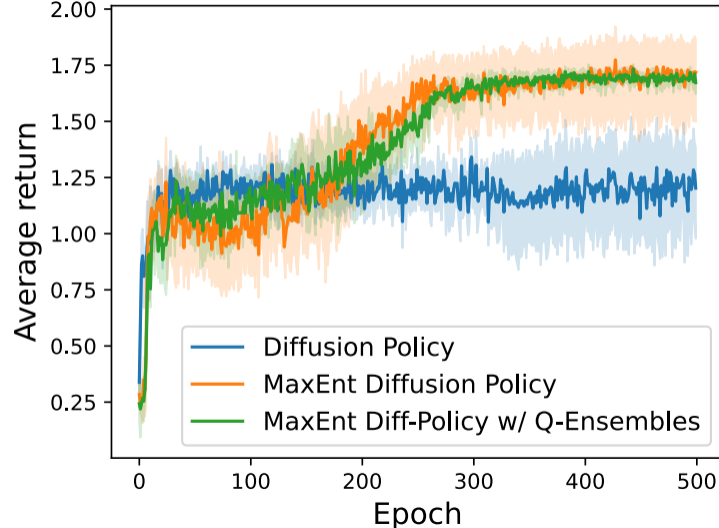
Training curves
