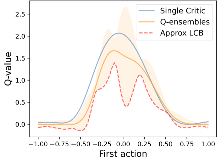
Learned Q-functions
